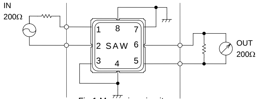
Fig.1 Measuring circuit
